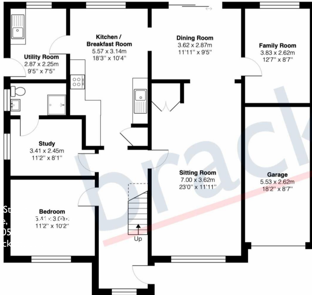
Ground Floor Approx 115.6 m / 1244 sq ft (Including Garage)
